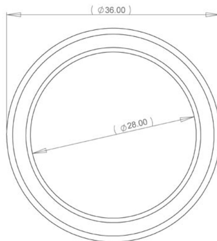
RB-RTA-30 (Retrofit Tank Adapter)
